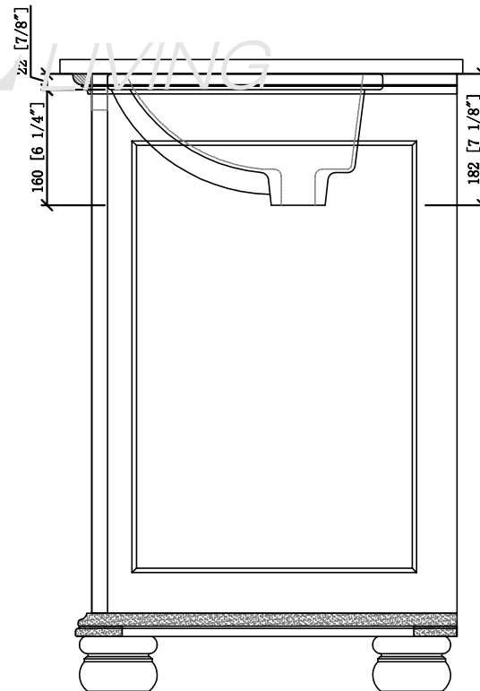
Platteville -30"Vanity combo drawing
