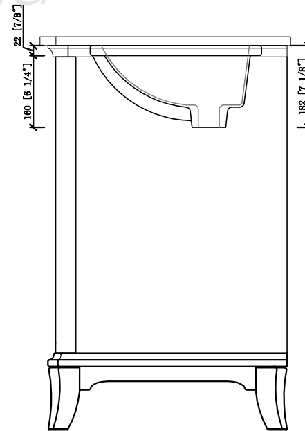
Rawsonville -48"Vanity combo drawing
